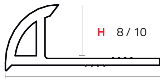
Chiusura perimetrale a muro/ Wall covering edging
