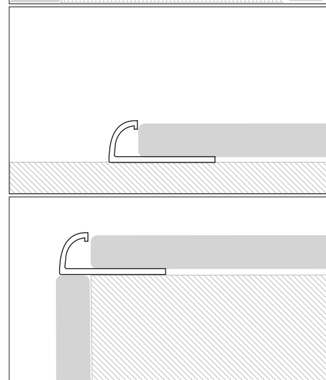
Chiusura perimetrale a muro/ Wall covering edging
