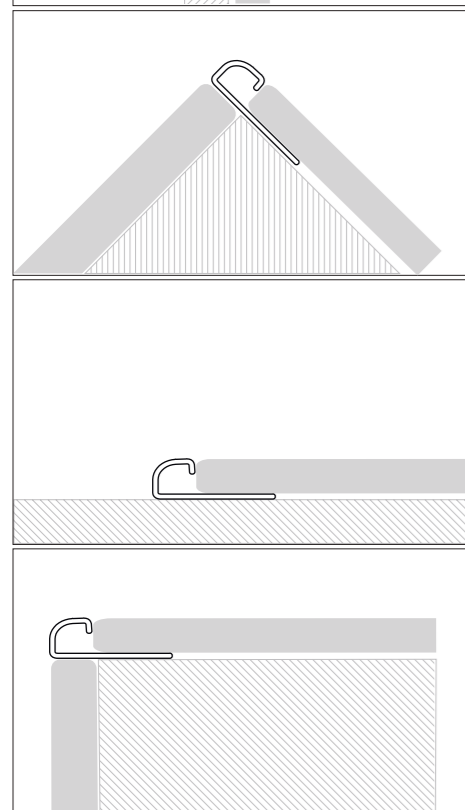
Chiusura perimetrale a muro/ Wall covering edging
