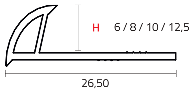
Chiusura perimetrale a muro/ Wall covering edging
