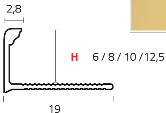
Chiusura perimetrale a muro/ Wall covering edging
